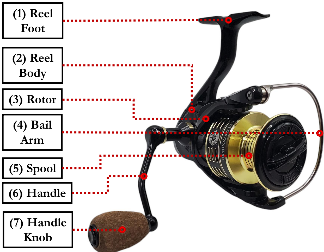
Figure 1: Reel Parts Diagram 1
